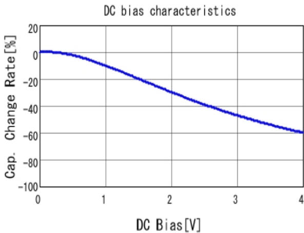
■ GRM188R60G106ME47 C-DC bias capchange, 25.0degC, AC0.
