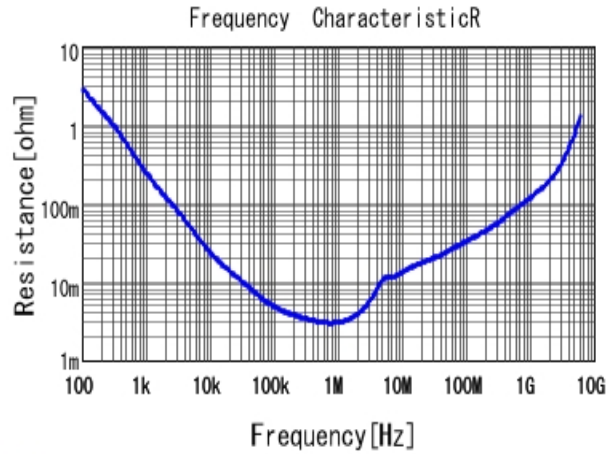
■ GRM188R60G106ME47 R DCOV, 25degC
