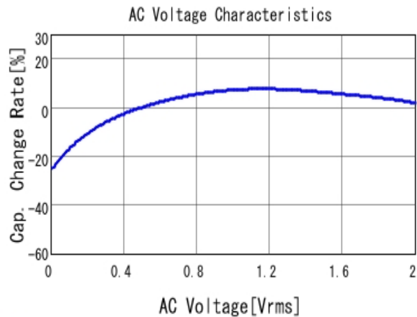
■ GRM188R60G106ME47 C-AC Voltage capchange, DCOV, 25.0d
