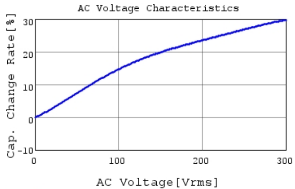
DE2B3SA471KN3AX02F C-AC Voltage capchange, I
