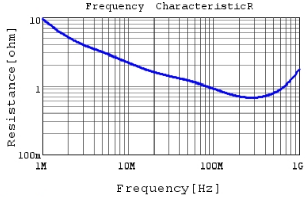
DE2B3SA471KN3AX02F R DCOV, 20degC
