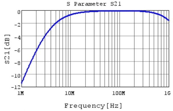
DE2B3SA471KN3AX02F S21 DCOV, 20degC
