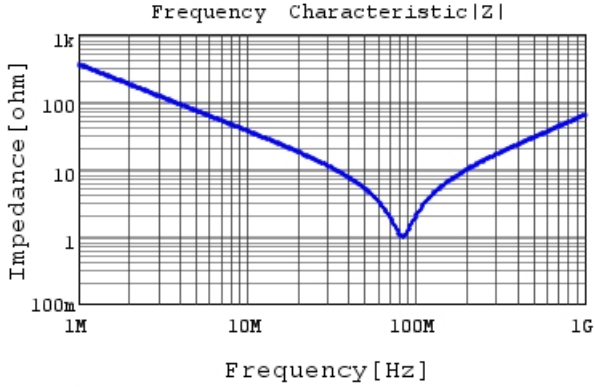
DE2B3SA471KN3AX02F |Z| DCOV, 20degC
