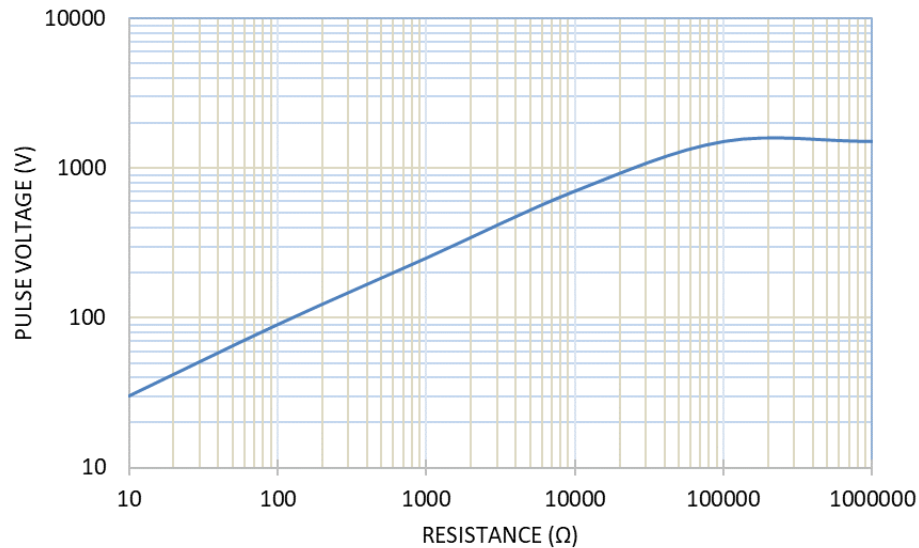
MLFA13 10/700 \mu s LIGHTNING SURGE
