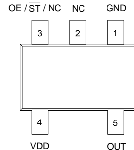
Figure 1. Pin Assignments
