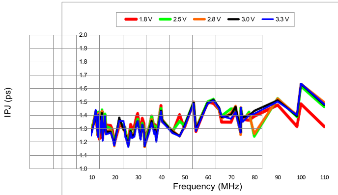
Figure 14. RMS Integrated Phase Jitter Random (12k to 20 MHz) vs Frequency [9]
