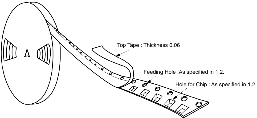
Fig.3 Taping Diagram
