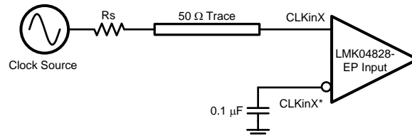
Figure 19. DC-Coupled LVCMOS/LVTTL Reference Clock
