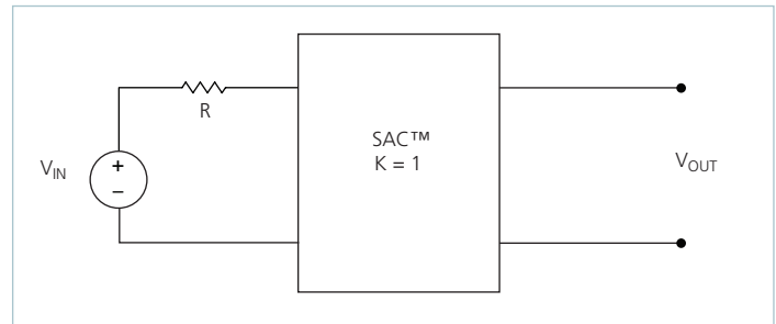
Figure 17 — K = 1 Sine Amplitude Converter with series input resistor
