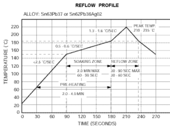
Figure 36. Reflow Profile.
