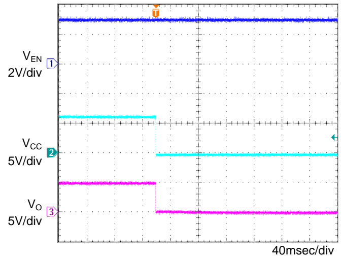
Figure 12. OFF sequence 1 Co=1 \mu F, Ta=-40°C
