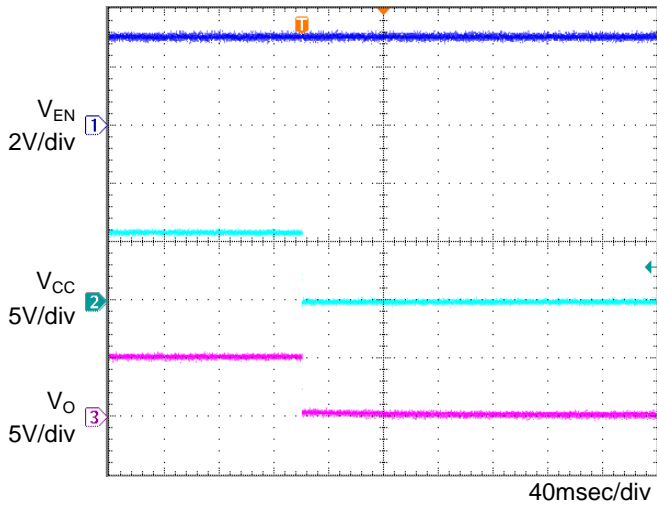
Figure 13. OFF sequence 1 Co=1 \mu F, Ta=25°C
