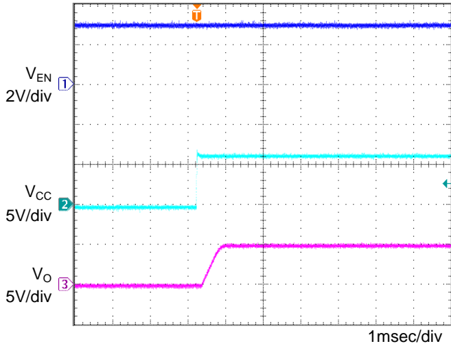
Figure 11. Input sequence 1 Co=1 \mu F, Ta=105°C
