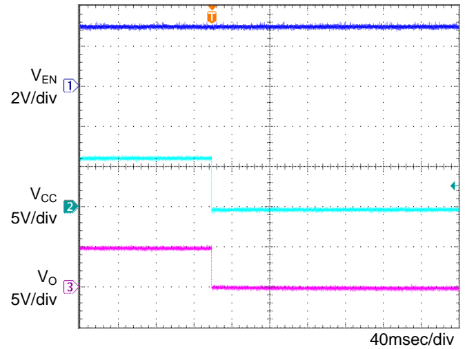
Figure 14. OFF sequence 1 Co=1 \mu F, Ta=105°C
