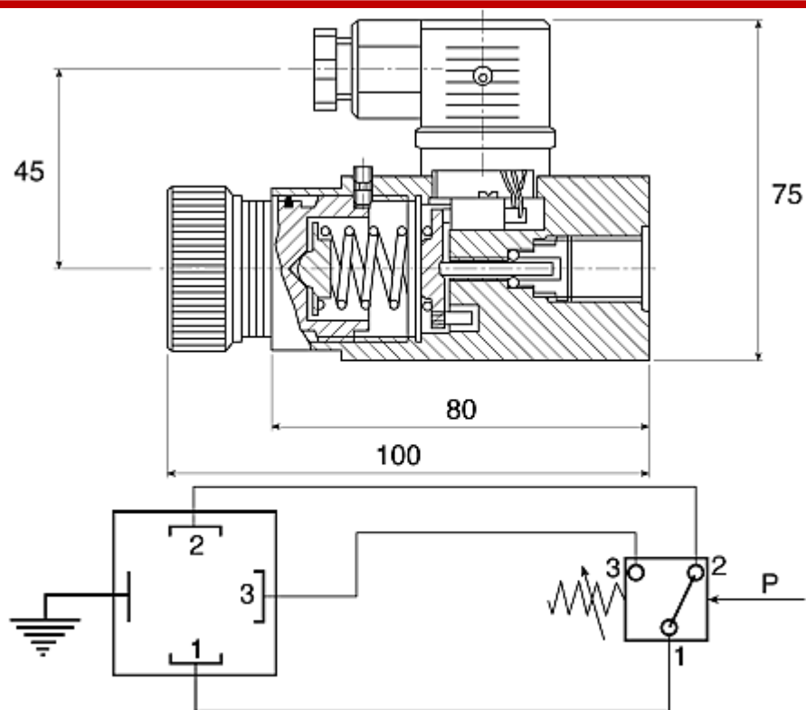
Electrical Connection
