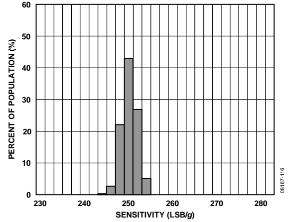
Figure 19. X-Axis Sensitivity at 25°C, V_s = 1.8\text{ V} , Full Resolution
