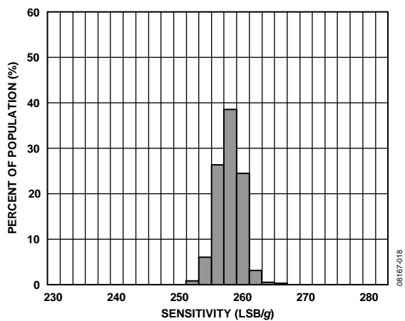
Figure 18. Z-Axis Sensitivity at 25°C, V_s = 2.6\text{ V} , Full Resolution
