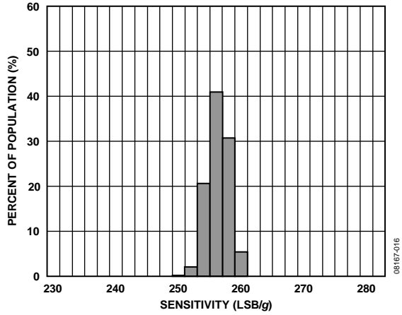
Figure 16. X-Axis Sensitivity at 25°C, V_s = 2.6\text{ V} , Full Resolution
