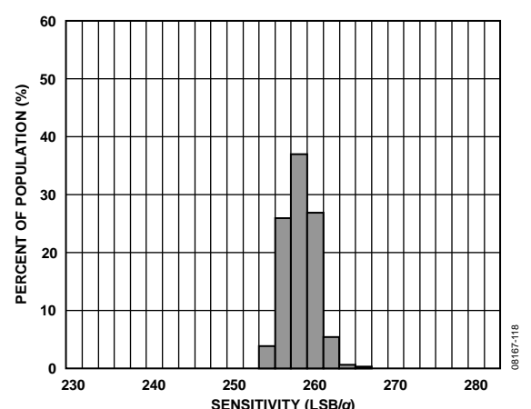
Figure 21. Z-Axis Sensitivity at 25°C, V_s = 1.8\text{ V} , Full Resolution
