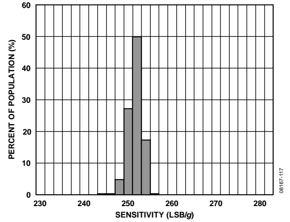
Figure 20. Y-Axis Sensitivity at 25°C, V_s = 1.8\text{ V} , Full Resolution
