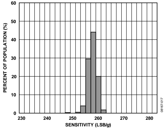
Figure 17. Y-Axis Sensitivity at 25°C, V_s = 2.6\text{ V} , Full Resolution
