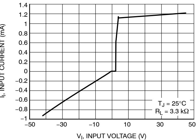
Figure 16. Input Current vs. Input Voltage
