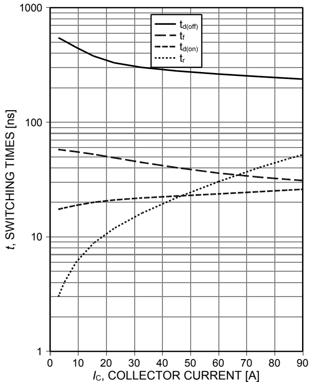
Figure 7. Typical switching times as a function of collector current (inductive load, T_{vj}=175^{\circ}C , V_{CE}=400V , V_{GE}=15/0V , r_G=10\Omega , Dynamic test circuit in Figure E)
