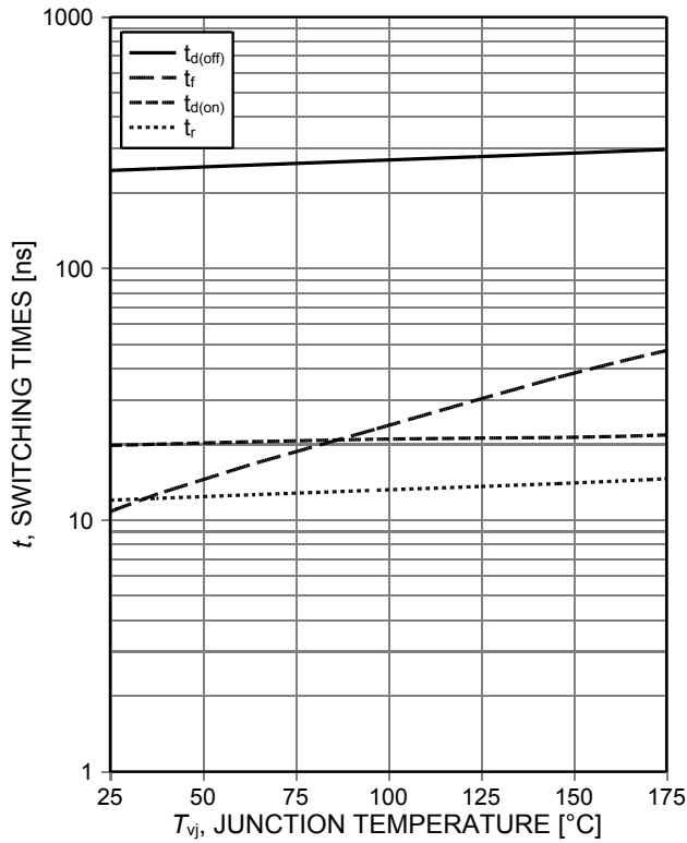
Figure 9. Typical switching times as a function of junction temperature (inductive load, V_{CE}=400V , V_{GE}=15/0V , I_C=30A , r_G=10\Omega , Dynamic test circuit in Figure E)
