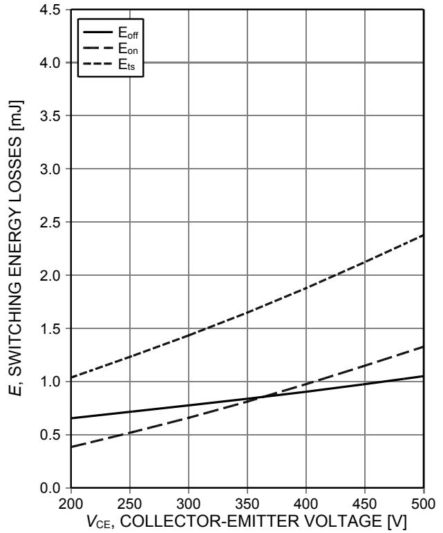
Figure 14. Typical switching energy losses as a function of collector emitter voltage (inductive load, T_{vj}=175^\circ C , V_{GE}=15/0V , I_C=30A , r_G=10\Omega , Dynamic test circuit in Figure E)
