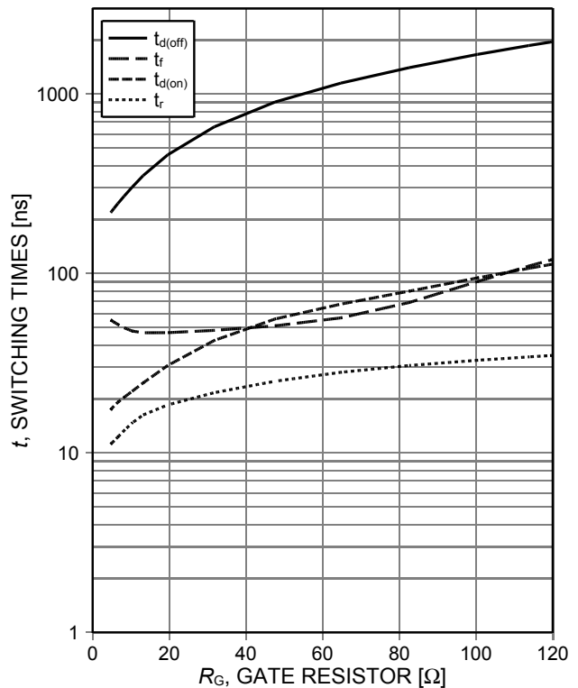
Figure 8. Typical switching times as a function of gate resistor (inductive load, T_{vj}=175^{\circ}C , V_{CE}=400V , V_{GE}=15/0V , I_C=30A , Dynamic test circuit in Figure E)
