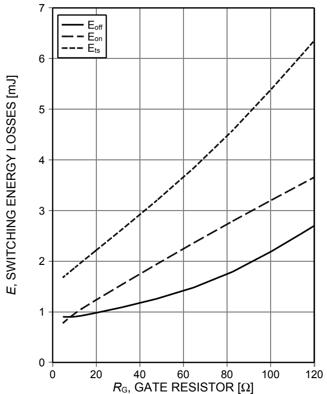
Figure 12. Typical switching energy losses as a function of gate resistor (inductive load, T_{vj}=175^\circ C , V_{CE}=400V , V_{GE}=15/0V , I_C=30A , Dynamic test circuit in Figure E)
