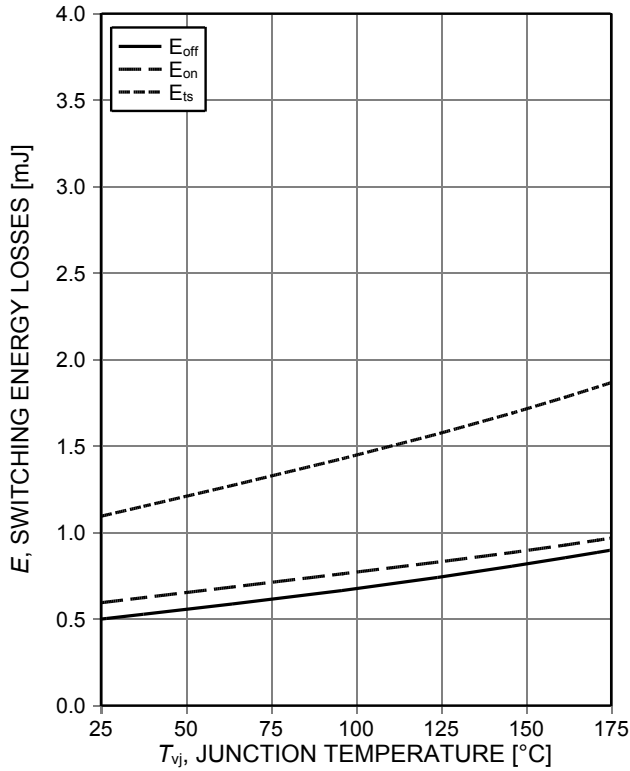
Figure 13. Typical switching energy losses as a function of junction temperature (inductive load, V_{CE}=400V , V_{GE}=15/0V , I_C=30A , r_G=10\Omega , Dynamic test circuit in Figure E)
