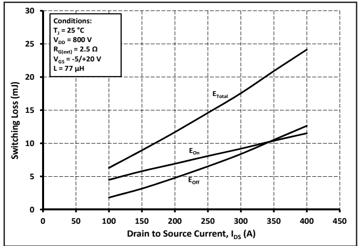
Figure 20. Inductive Switching Energy vs. Drain Current For V_{DS} = 800\text{V} , R_G = 2.5\ \Omega
