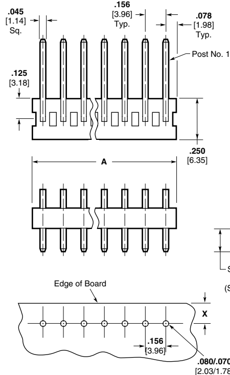
Recommended Mounting Hole Pattern for .062 [1.57] Thk. PC Board
