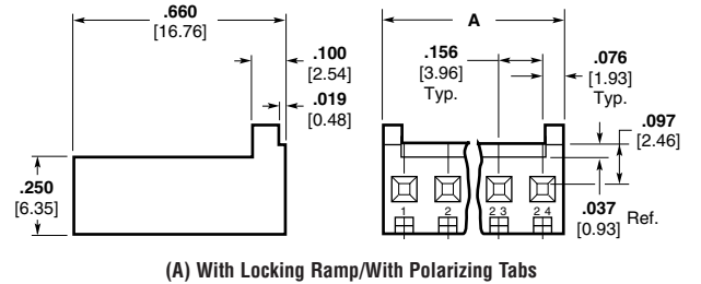
(A) With Locking Ramp/With Polarizing Tabs
