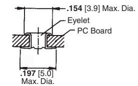
Soldering Side
