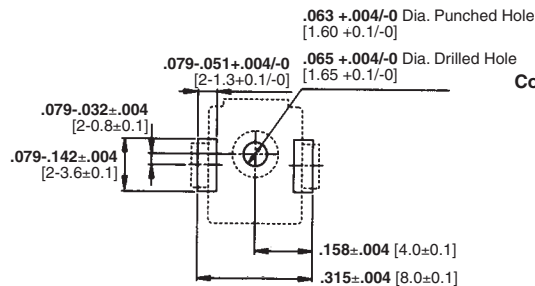
Recommended PC Board Layout Acceptable Board Thickness .062 [1.57]
