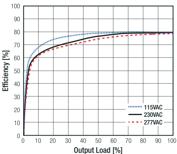
RAC04-12SK/277
