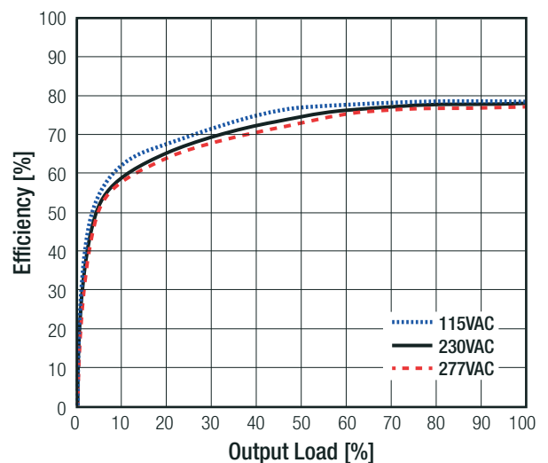
RAC04-15SK/277
