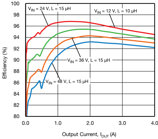
Fig. 23 - SiC463 Efficiency vs. Output Current, VOUT = 5 V
