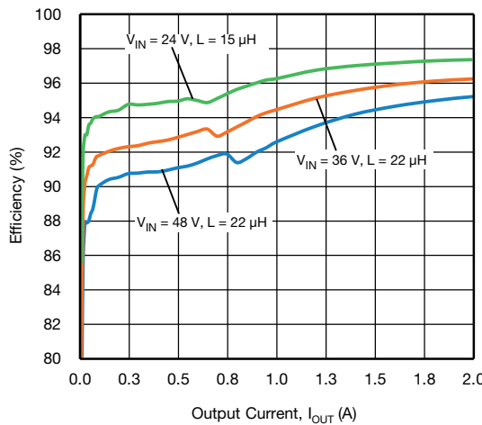
Fig. 30 - SiC464 Efficiency vs. Output Current, VOUT = 12 V
