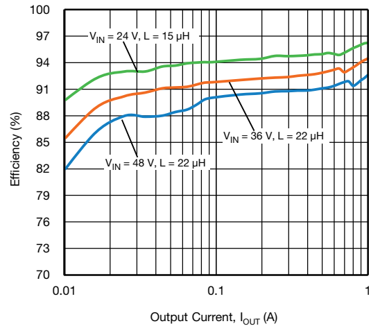
Fig. 27 - SiC463 Efficiency vs. Output Current - Light Load, VOUT = 12 V
