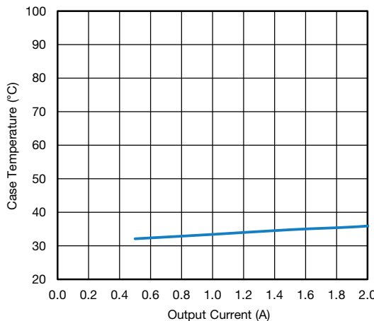
Fig. 31 - SiC464 Load Current vs. Case Temperature, VIN = 48 V, VOUT = 5 V
