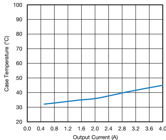
Fig. 25 - SiC463 Load Current vs. Case Temperature, VIN = 48 V, VOUT = 5 V
