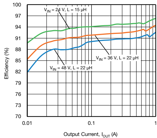
Fig. 33 - SiC464 Efficiency vs. Output Current - Light Load, VOUT = 12 V
