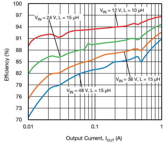
Fig. 32 - SiC464 Efficiency vs. Output Current - Light Load, VOUT = 5 V
