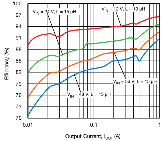
Fig. 26 - SiC463 Efficiency vs. Output Current - Light Load, VOUT = 5 V
