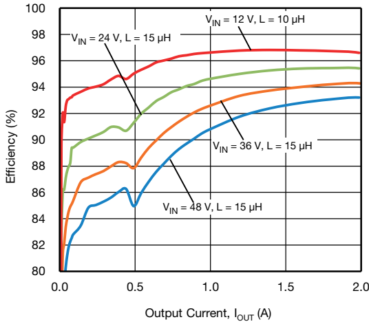
Fig. 29 - SiC464 Efficiency vs. Output Current, VOUT = 5 V
