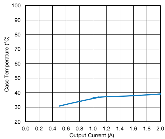
Fig. 34 - SiC464 Load Current vs. Case Temperature, VIN = 48 V, VOUT = 12 V
