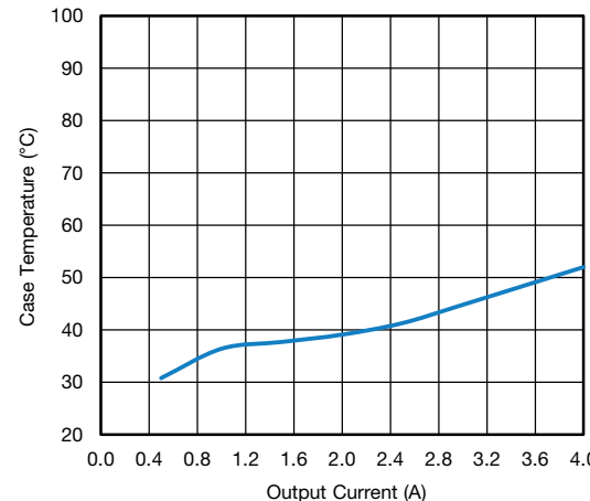
Fig. 28 - SiC463 Load Current vs. Case Temperature, VIN = 48 V, VOUT = 12 V
