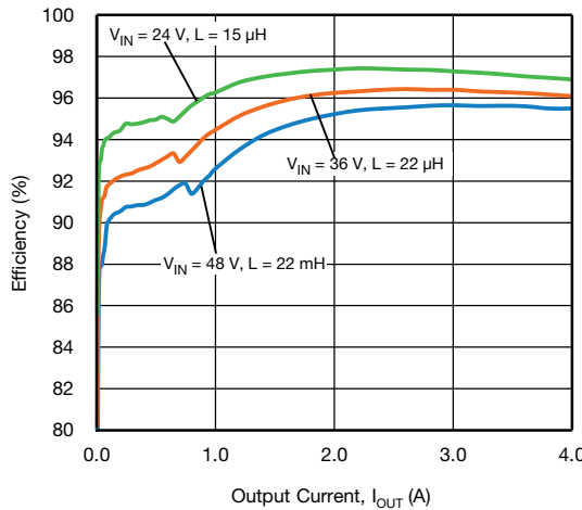
Fig. 24 - SiC463 Efficiency vs. Output Current, VOUT = 12 V
