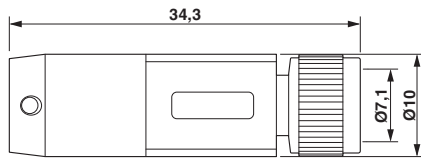
Dimensioned drawing
