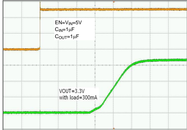
Start-up Time
