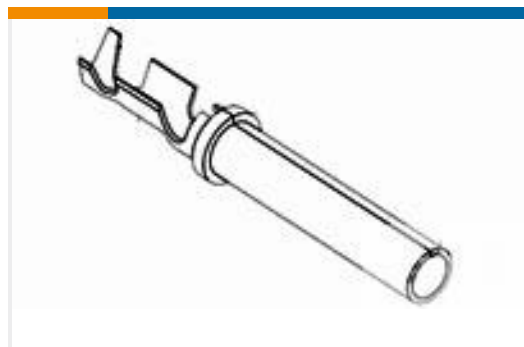
TE Part #1924464-2 SOC, SF, SIZE 16, 18-20 AWG, NI/SN
