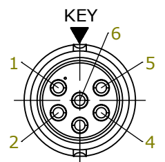
WIRING END W6282-6PG-P-5XX
