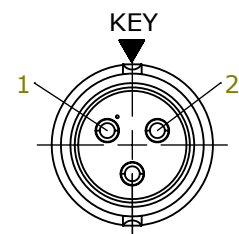
WIRING END W6282-3PG-P-5XX
