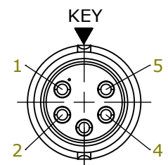
WIRING END W6282-5PG-P-5XX
