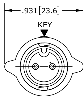
MATING FACE ASSY: W6282-2PG-P-5XX SHOWN
