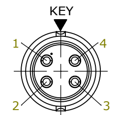
WIRING END W6282-4PG-P-5XX
