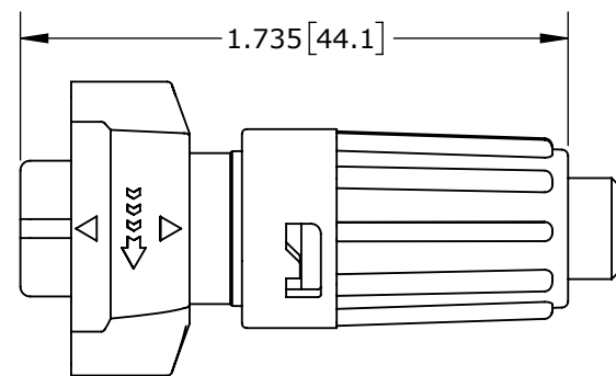
SHOWN ASSEMBLED KIT ASSY: W6282-2PG-P-5XX SHOWN
