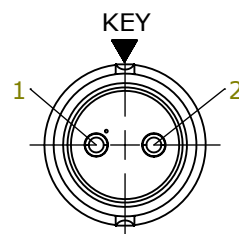
WIRING END W6282-2PG-P-5XX
