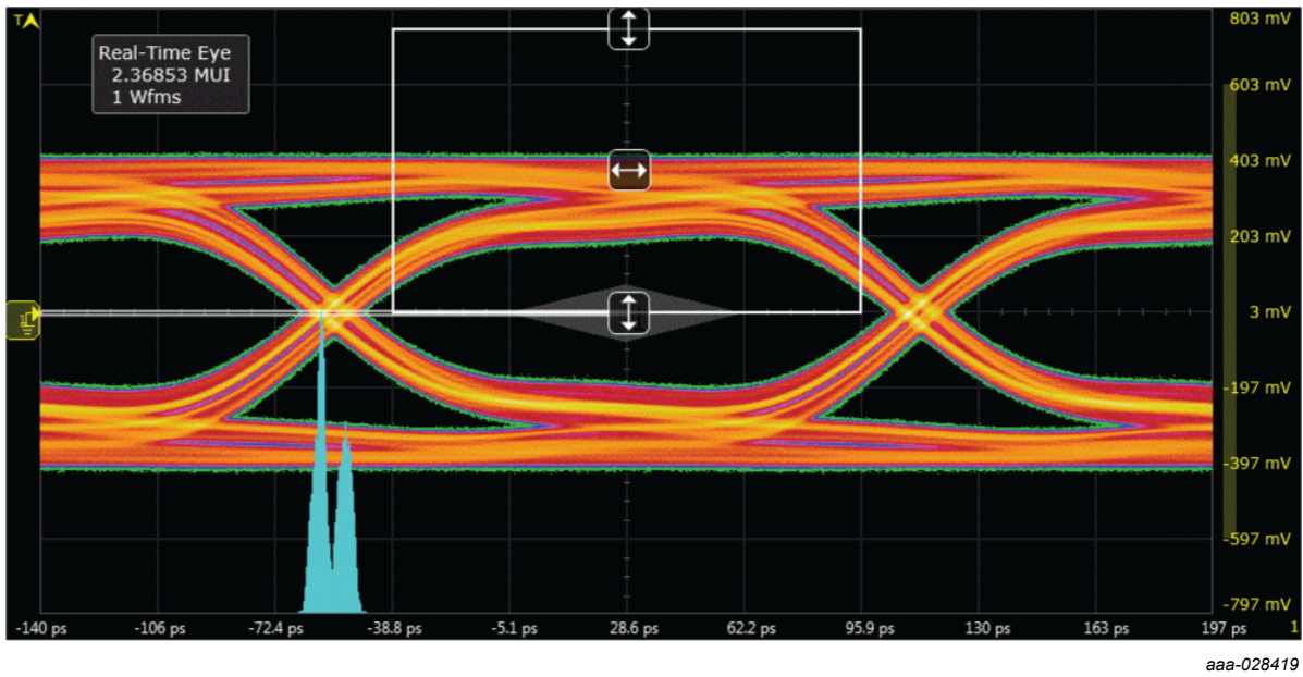
Fig. 6. HDMI TP1 eye diagram, PCB with device; typical values
