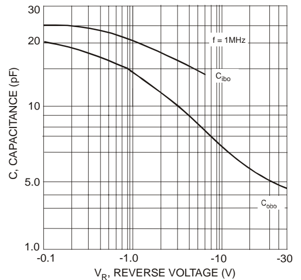
Fig. 16, Typical Capacitance (DRDP006W)
