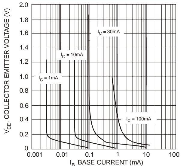
Fig. 6, Typical Collector Saturation Region (DRDN005W)
