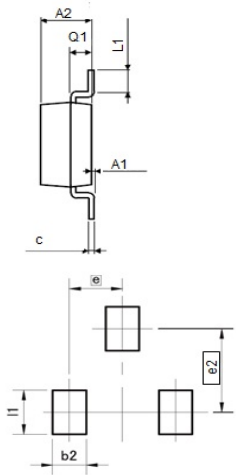
Pattern of terminal position areas [Not a pattern of soldering pads]
