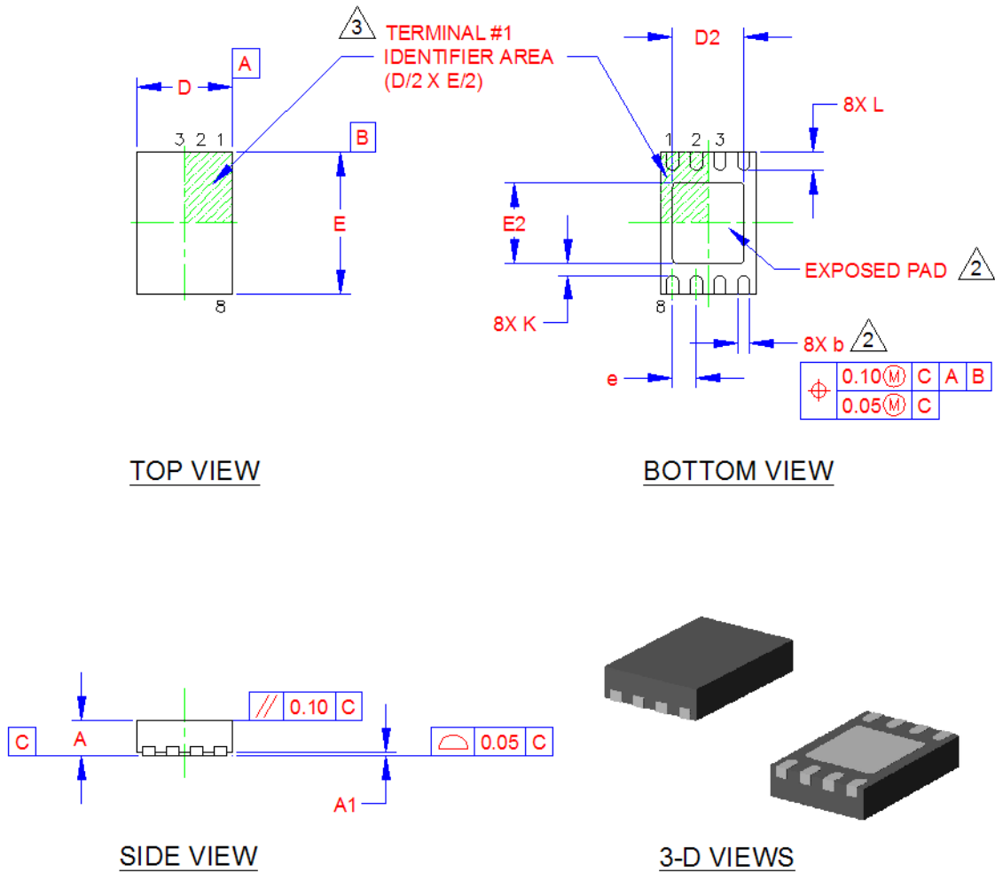
Figure 2 EMC1412 2mm x 3mm TDFN Package Drawing
