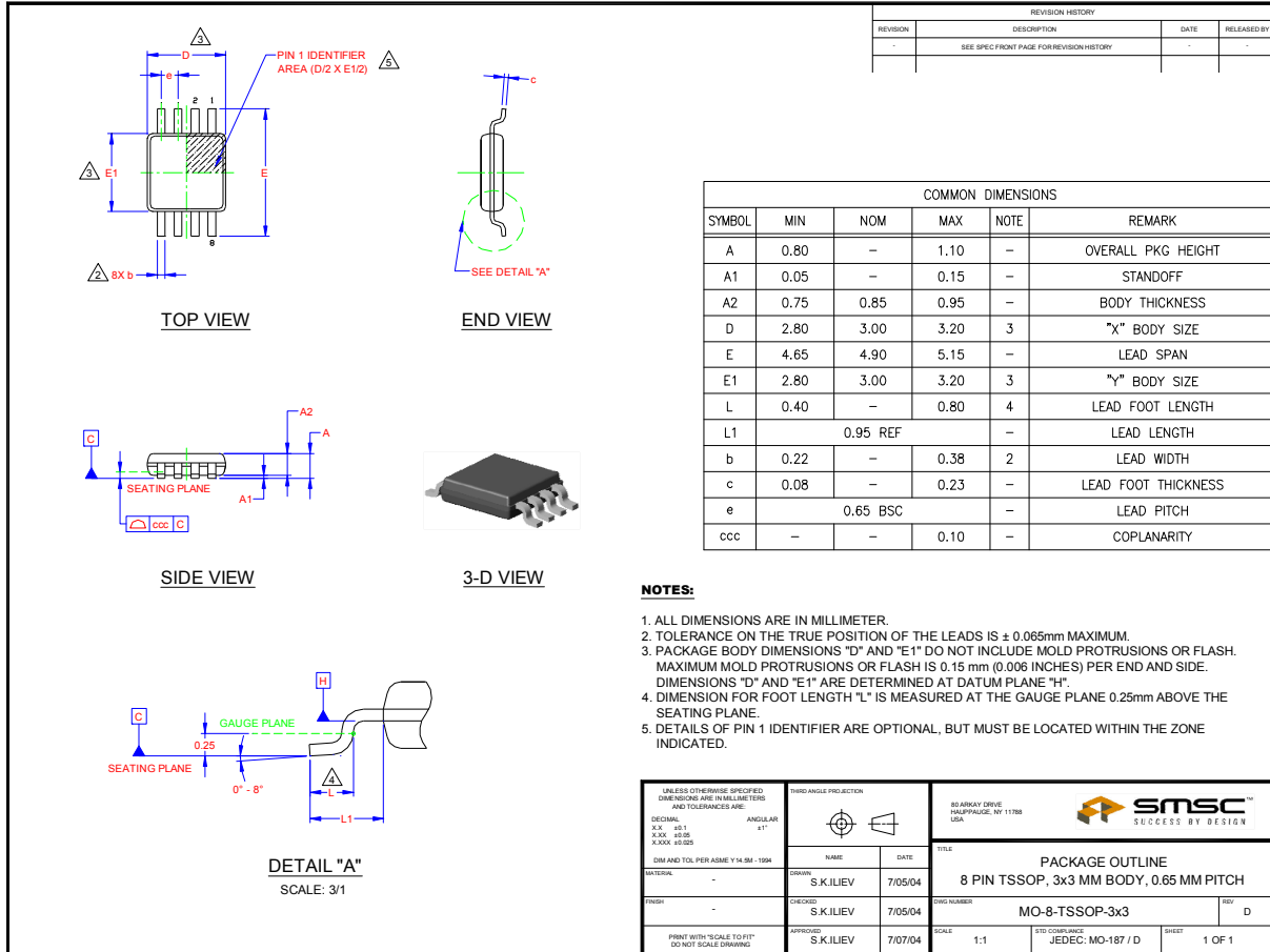
Figure 5 8-Pin MSOP / TSSOP Package
