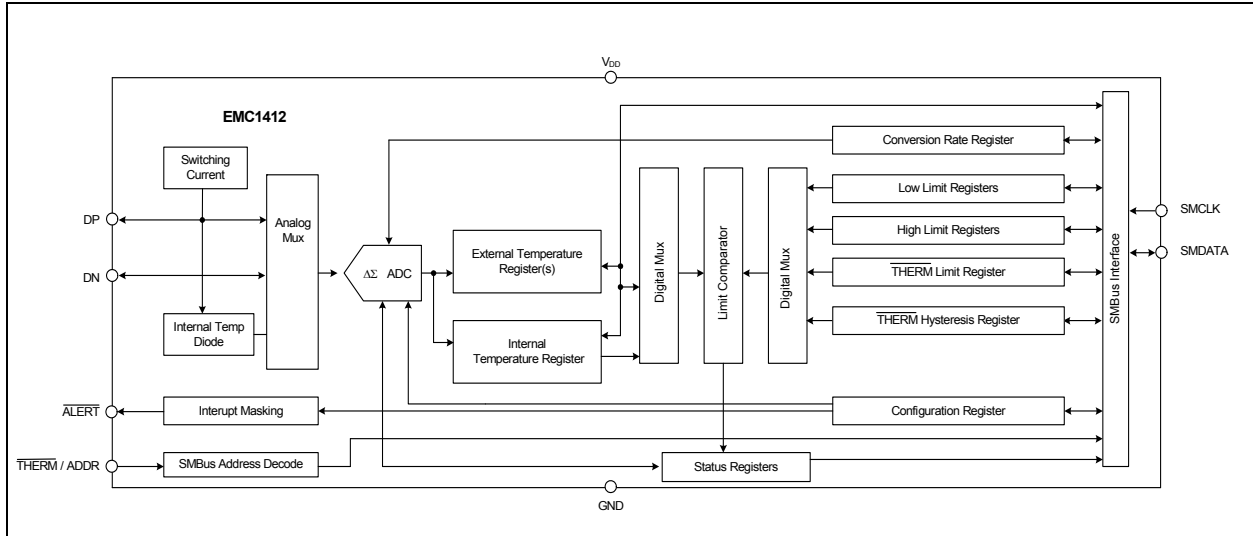
Figure 1 EMC1412 Block Diagram
