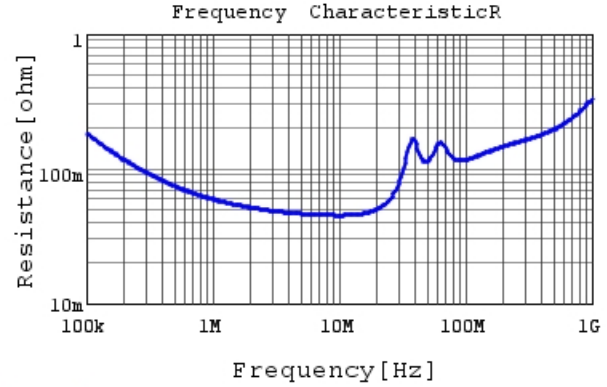
RDER72J104K4M1H03A R DCOV,25degC
