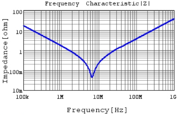
RDER72J104K4M1H03A |Z| DCOV,25degC
