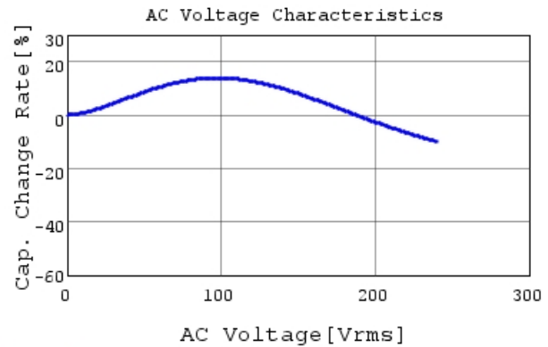
RDER72J104K4M1H03A C-AC Voltage capchange, I
