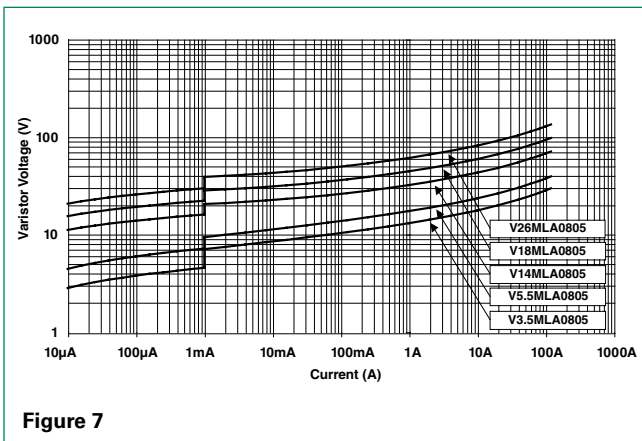
Limit V-I Characteristic for V3.5MLA0805 to V26MLA0805
