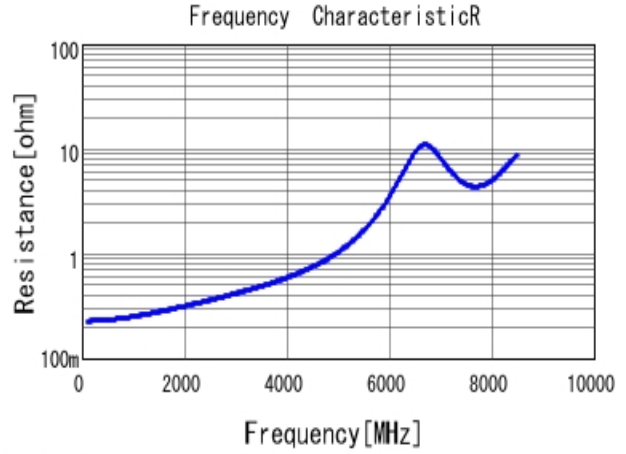
■ GCM1555C1H6R8FA16 R DCOV, 25degC
