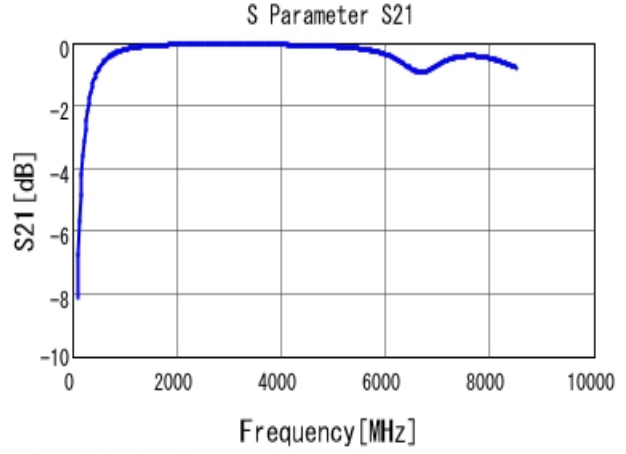
■ GCM1555C1H6R8FA16 S21 DCOV, 25degC
