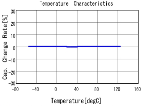
■ GCM1555C1H6R8FA16 C-Temp. capchange, DCOV, AC1Vrms
