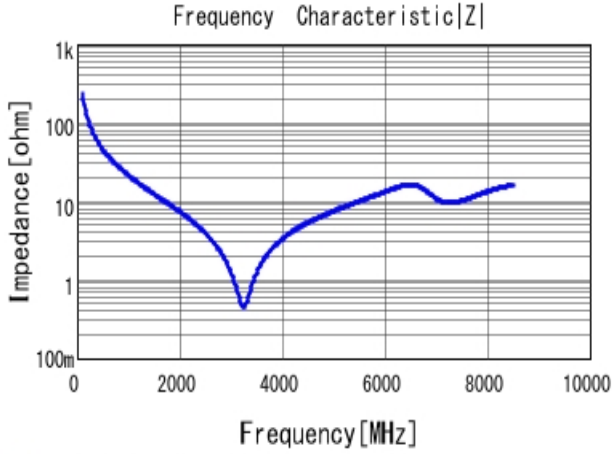
■ GCM1555C1H6R8FA16 |Z| DCOV, 25degC
