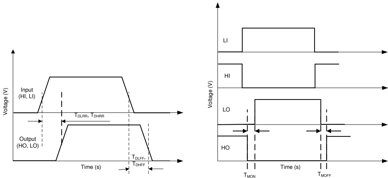
Figure 6-1. Timing Diagram
