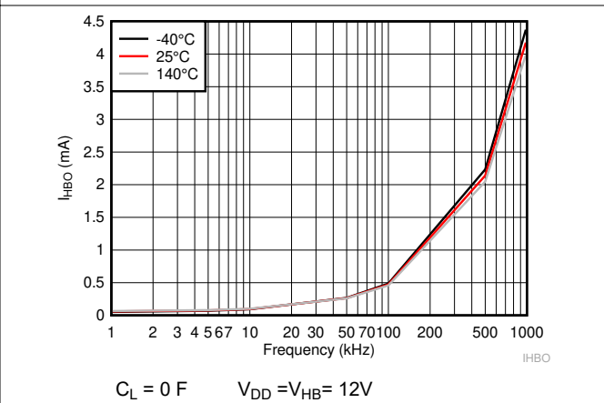
Figure 6-5. HB Operating Current
