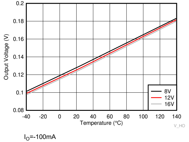
Figure 6-15. HO High Output Voltage ( V_{HOH} )
