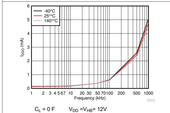
Figure 6-4. VDD Operating Current
