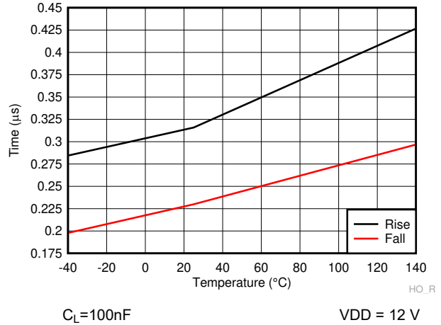
Figure 6-21. HO Rise & Fall Time
