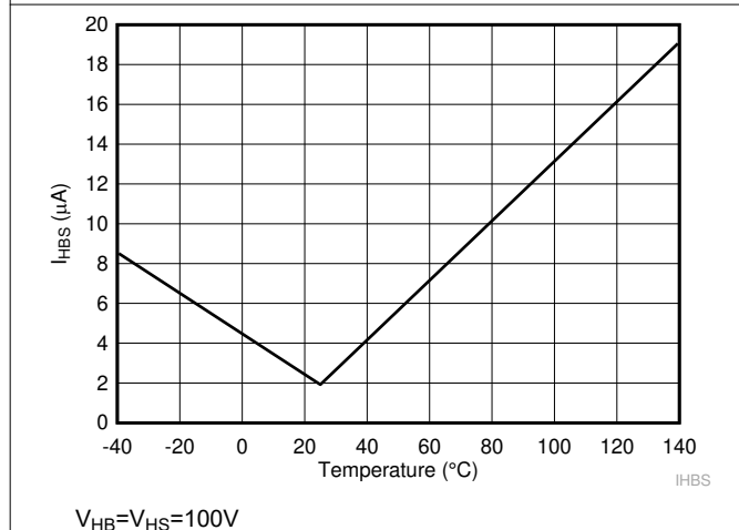
Figure 6-6. HB to VSS Quiescent Current
