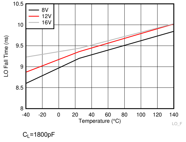
Figure 6-17. LO Fall Time
