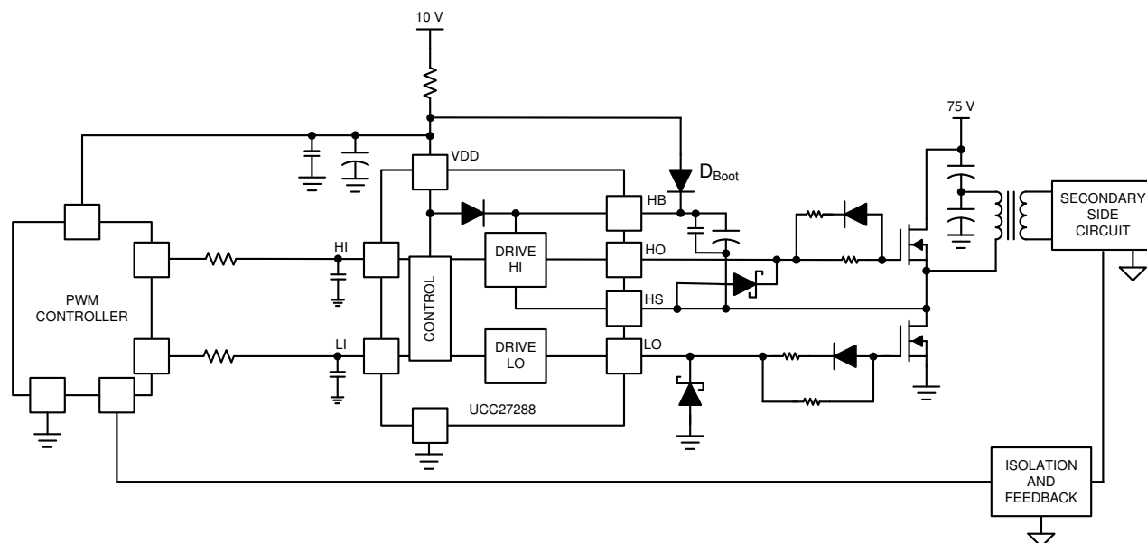
Figure 8-1. Typical Application
