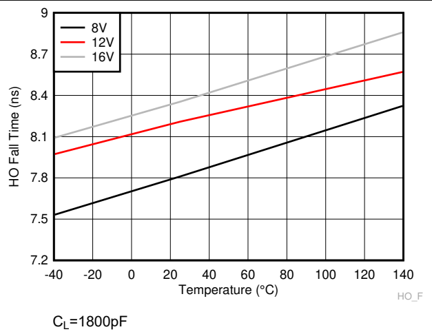
Figure 6-19. HO Fall Time
