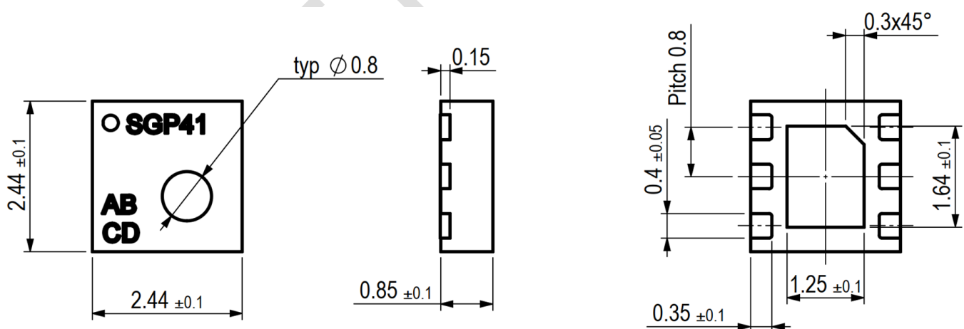
Figure 17 Package outline drawing of the SGP41. Dimensions are given in millimeters.
