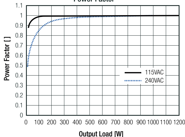
Power Factor
