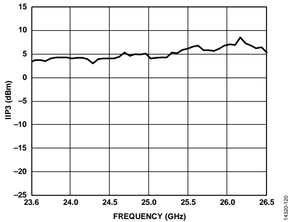
Figure 20. IIP3 vs. Frequency
