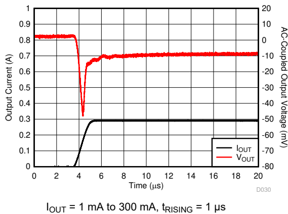
Figure 6-51. Load Transient
