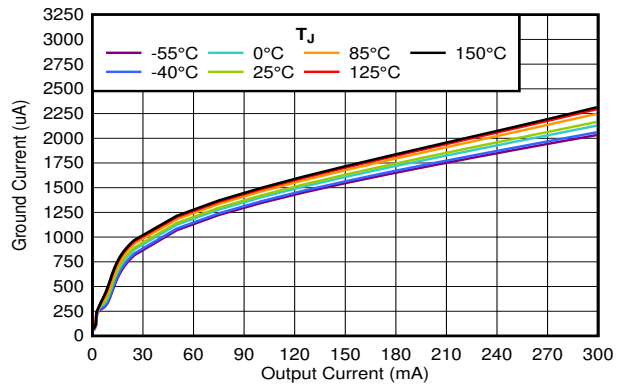
Figure 6-38. I_{GND} vs I_{OUT}
