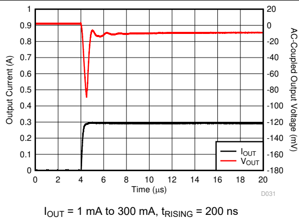
Figure 6-53. Load Transient
