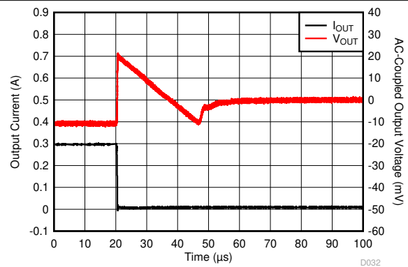
I_{OUT} = 300\text{ mA to }1\text{ mA} , t_{FALLING} = 200\text{ ns}
