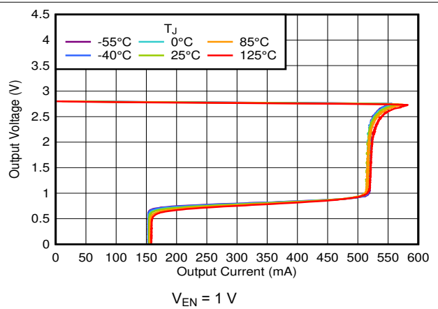
Figure 6-44. Current Limit
