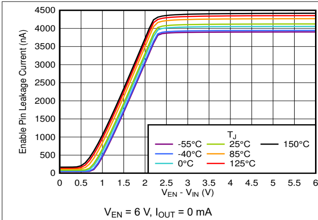
Figure 6-43. Enable Pin Leakage Current vs V_{EN} - V_{IN}
