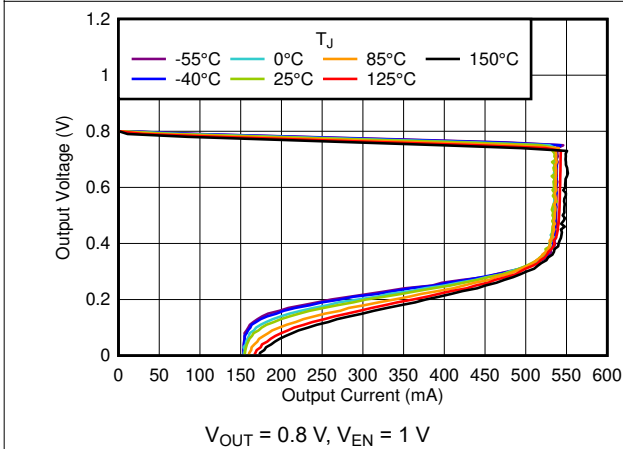
Figure 6-45. Current Limit
