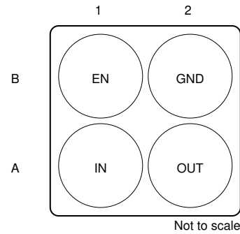
Figure 5-2. YCJ and YCK Packages (Preview), 4-Pin DSBGA, Bottom View
