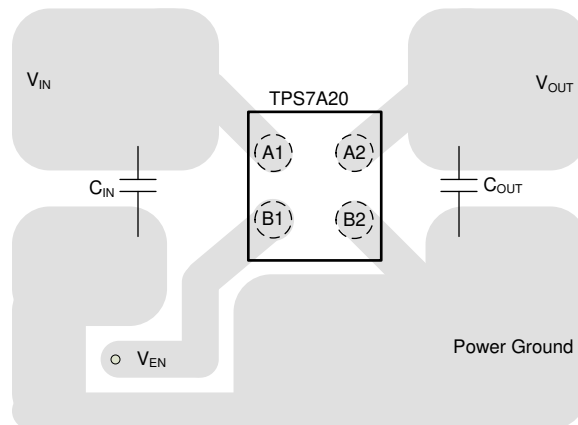
Figure 10-3. YCK Package (DSBGA) Typical Layout
