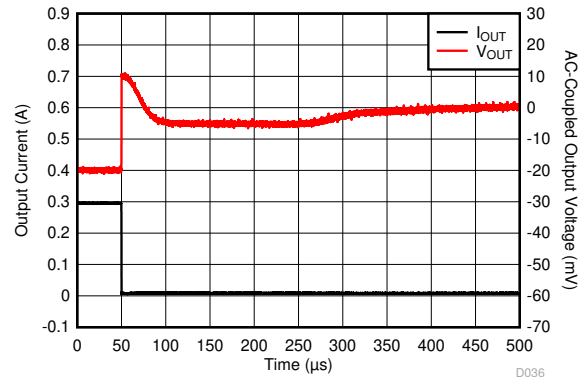
Figure 6-56. Load Transient
