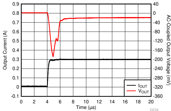
Figure 6-55. Load Transient
