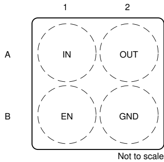
Figure 5-1. YCJ and YCK Packages (Preview), 4-Pin DSBGA, Top View
