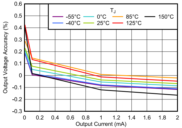
Figure 6-16. Output Voltage Accuracy vs I_{OUT}
