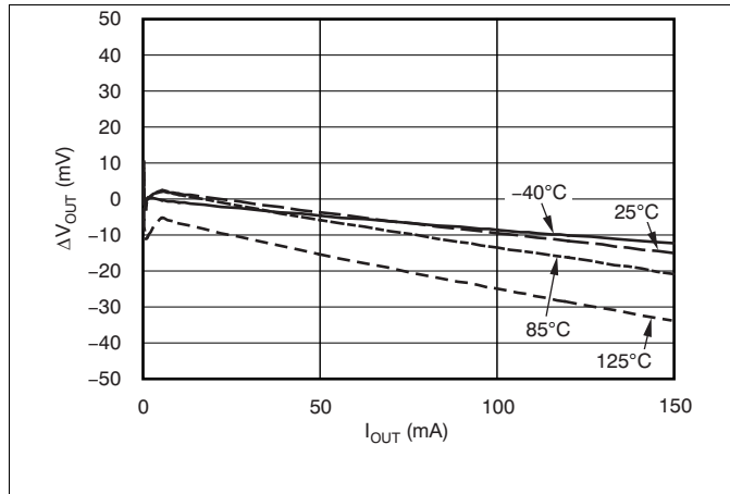
Figure 1. Load Regulation
