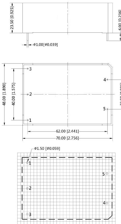
Note:Grid 2.54*2.54mm Recommended PCB Layout Top View
