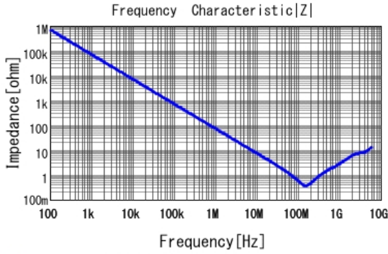
■ GCJ188R71H222KA01 |Z| DCOV, 25degC
