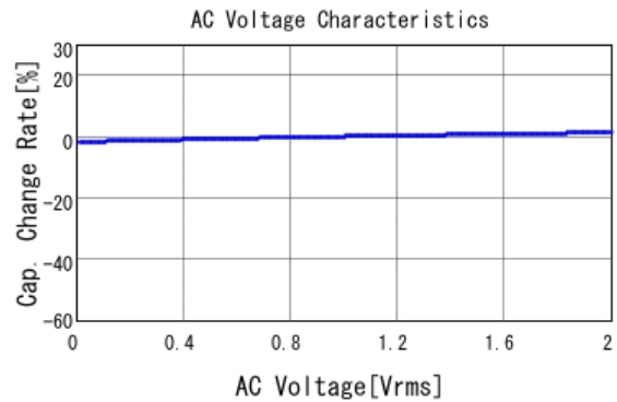
■ GCJ188R71H222KA01 C-AC Voltage capchange, DCOV, 25.0d
