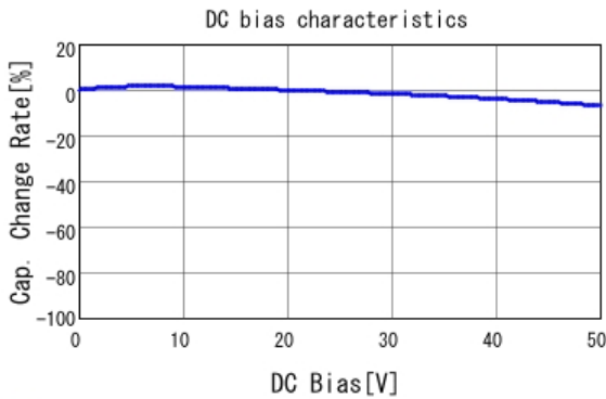
■ GCJ188R71H222KA01 C-DC bias capchange, 25.0degC, AC1.
