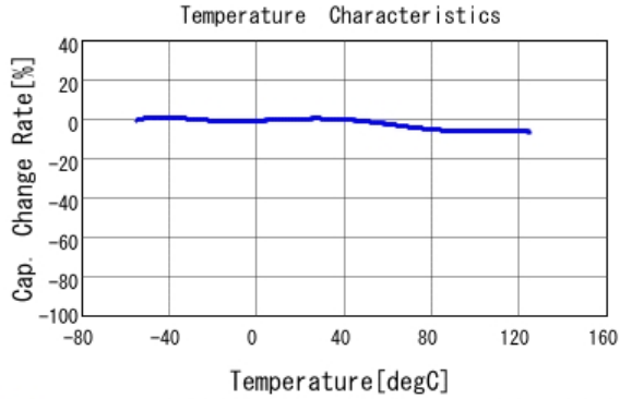
■ GCJ188R71H222KA01 C-Temp. capchange, DC0.0V, AC1.0Vrm
