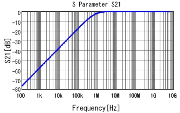
■ GCJ188R71H222KA01 S21 DC0V, 25degC
