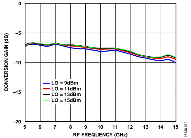
Figure 50. Conversion Gain vs. RF Frequency at Various LO Power Levels, T_A = 25^\circ\text{C}
