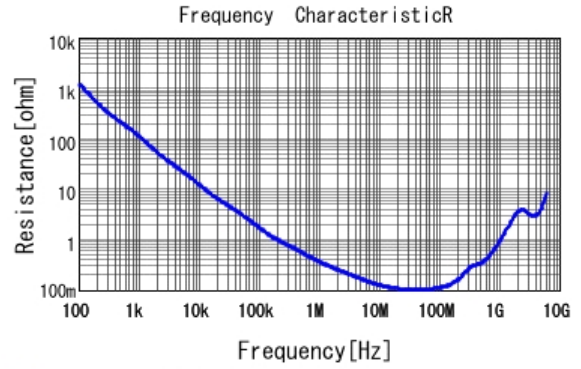
GCM188R72A682KA37 R DCOV, 25degC
