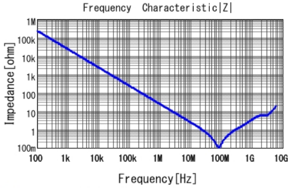
GCM188R72A682KA37 |Z| DCOV, 25degC
