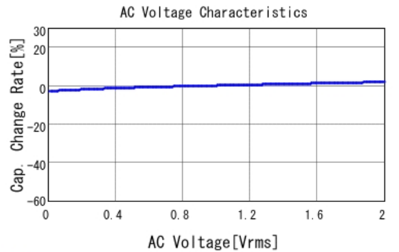
GCM188R72A682KA37 C-AC Voltage capchange, DCOV, 25.0d
