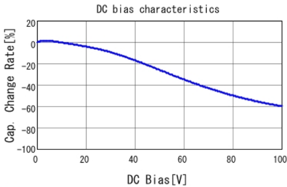
GCM188R72A682KA37 C-DC bias capchange, 25.0degC, AC1.
