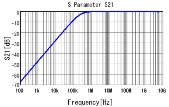
■ GCM188R72A682KA37 S21 DC0V, 25degC
