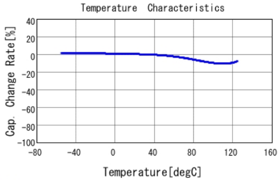
■ GCM188R72A682KA37 C-Temp. capchange, DC0.0V, AC1.0V rm
