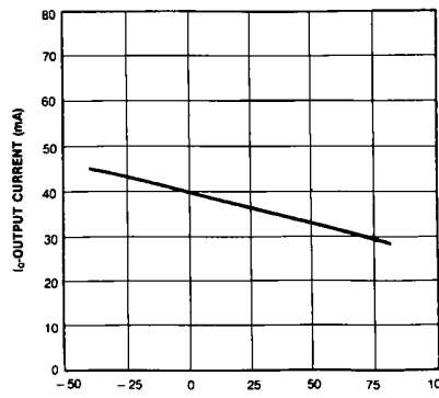
Figure 11. Current Limiting vs Temperature
