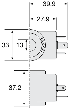
Dimensions (mm)
