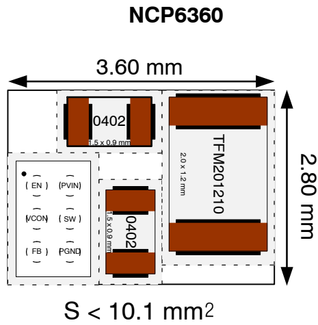
Figure 39. Layout Minimum Recommended Occupied Space Using 0402 Capacitors and 0805 (2.0 x 1.2 x 1 mm) Inductor
