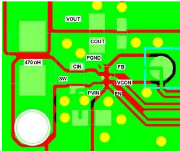
Figure 40. Example of PCB Implementation (PCB case with 0805 (2.0x1.2 mm) Capacitors and 2016 (2.0 x 1.6 x 1 mm) Inductors)
