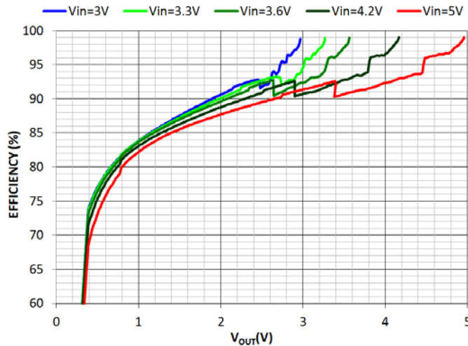
Figure 20. Efficiency vs. V_{OUT} R_L = 22\ \Omega , Temp = 25^\circ\text{C}
