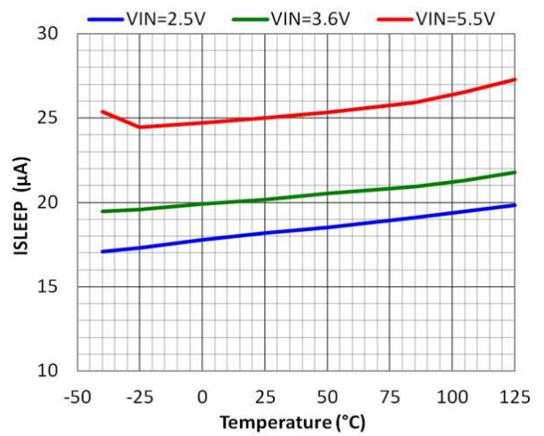
Figure 7. Sleep Mode Current vs. Temperature (EN = High, VCON = 0 V, V_{OUT} = 0\text{ V} )
