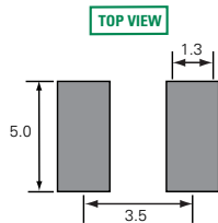
Recommended Soldering Pad Layout
