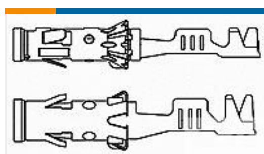
TE Part # CAT-R7602-T273 ROUND CONNECTOR SYSTEM, PIN AND SOCKET
