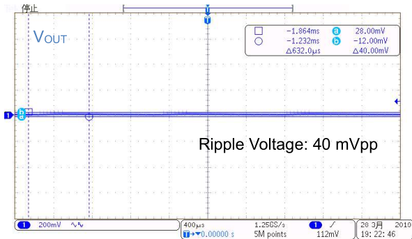
Figure 43. V_{IN} = 115 \text{ Vdc} , I_{OUT} = 10 \text{ mA}
