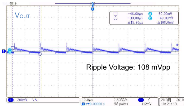
Figure 45. V_{IN} = 115 \text{ Vac} , I_{OUT} = 3.0 \text{ A}
