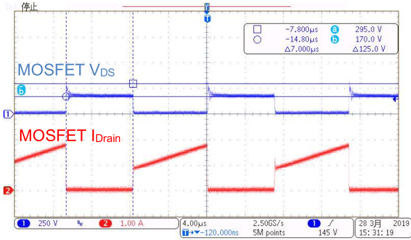
Figure 31. MOSFET V_{IN} = 90 \text{ Vac} , I_{OUT} = 4.0 \text{ A}
