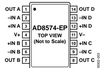
Figure 1. 14-Lead TSSOP
