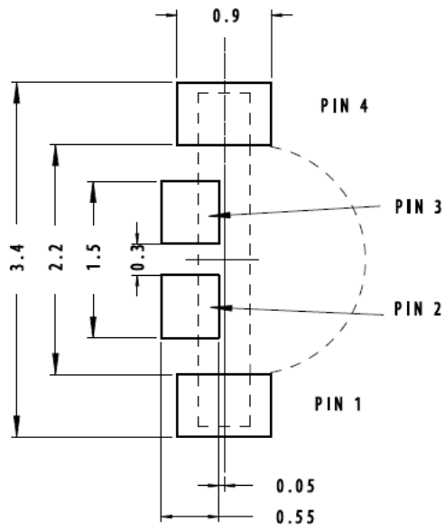
Figure 7: Recommended Soldering Land Pattern
