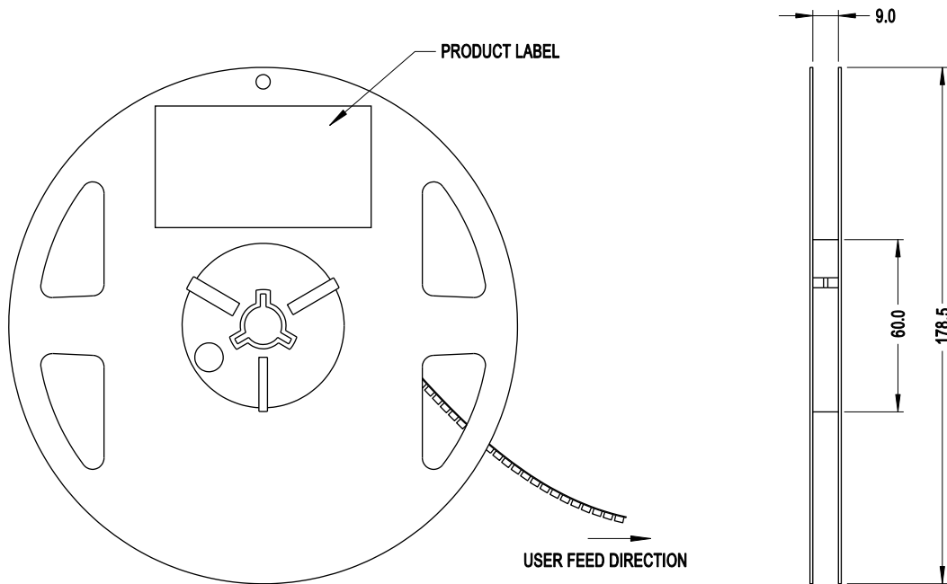
Figure 9: Reel Dimensions
