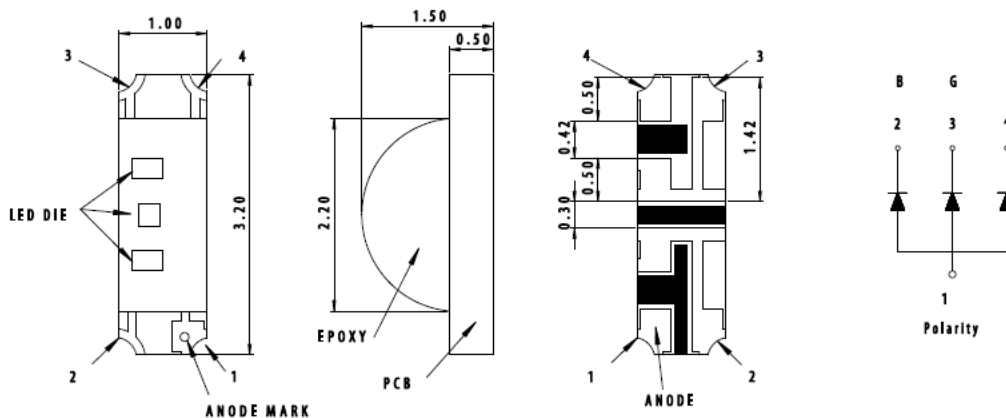
Figure 1: Package Dimensions
