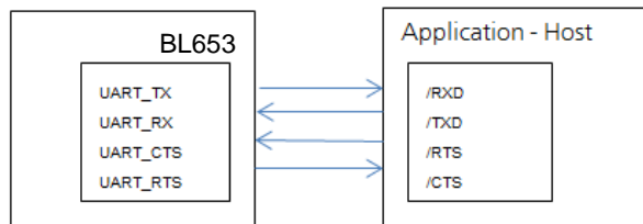
Figure 6: UART signals
