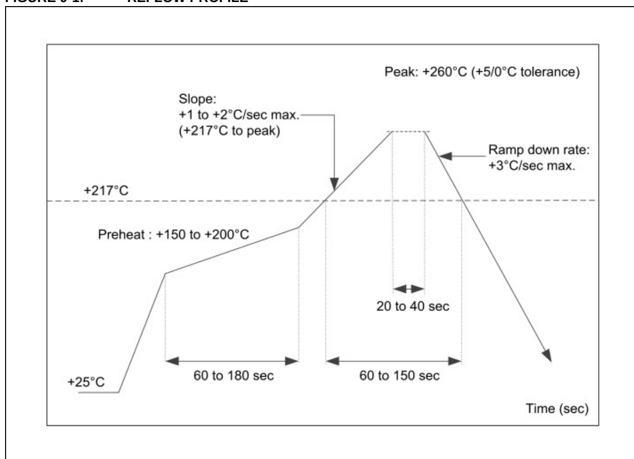
FIGURE 9-1: REFLOW PROFILE
