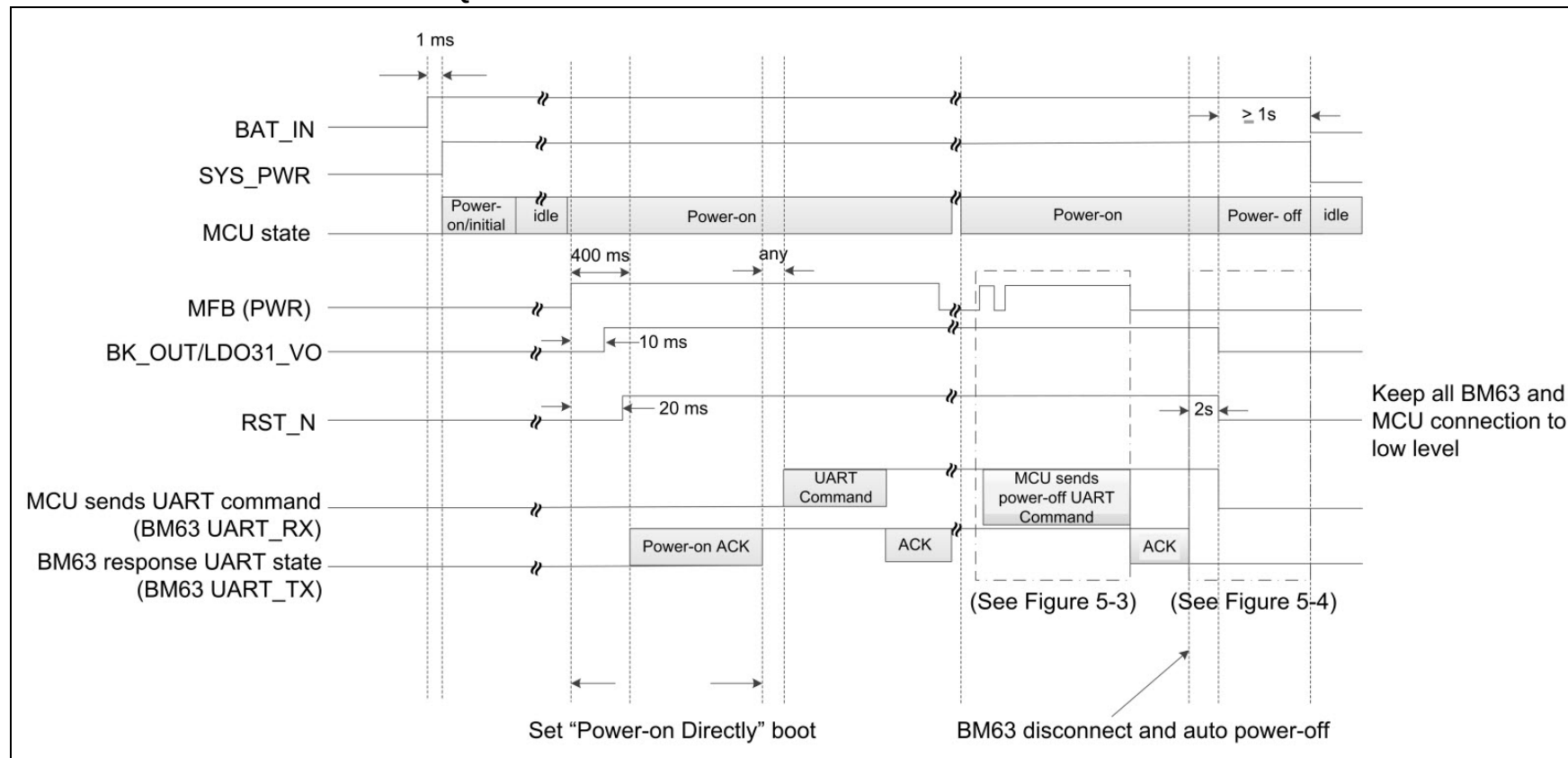
FIGURE 5-2: POWER-ON/OFF SEQUENCE
