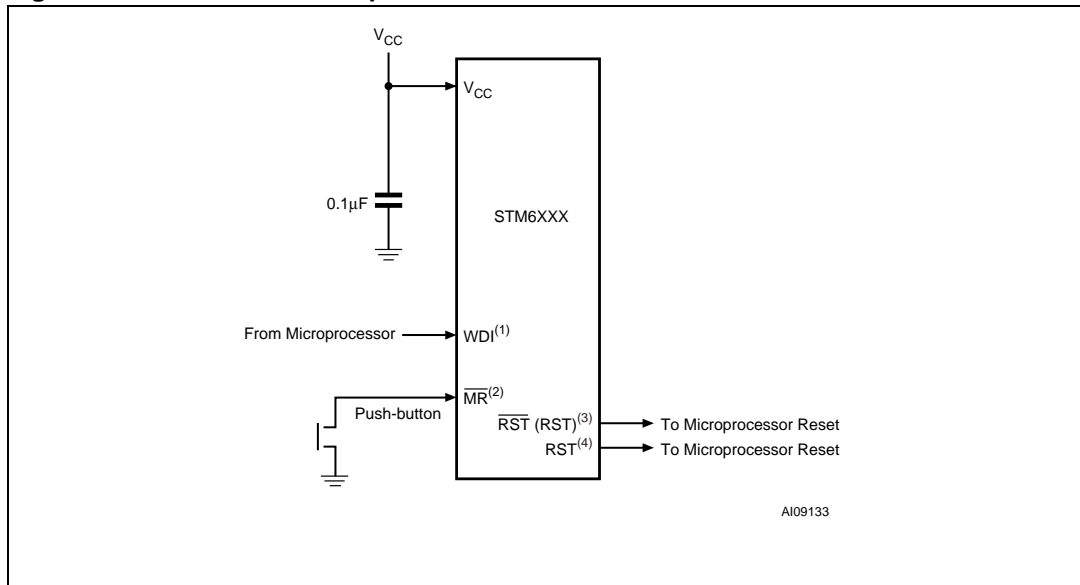
Figure 11. Hardware Hookup
