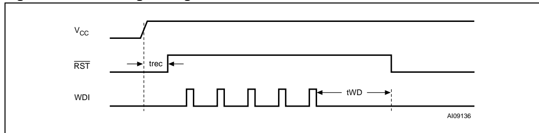
Figure 27. Watchdog Timing
