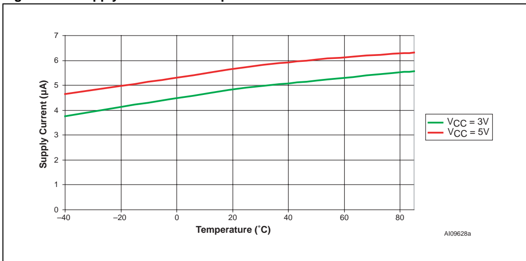
Figure 17. Supply Current vs. Temperature
